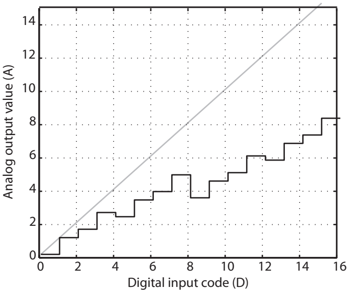
Figure 25. Input/output characteristics of a radix 1.5 DAC
