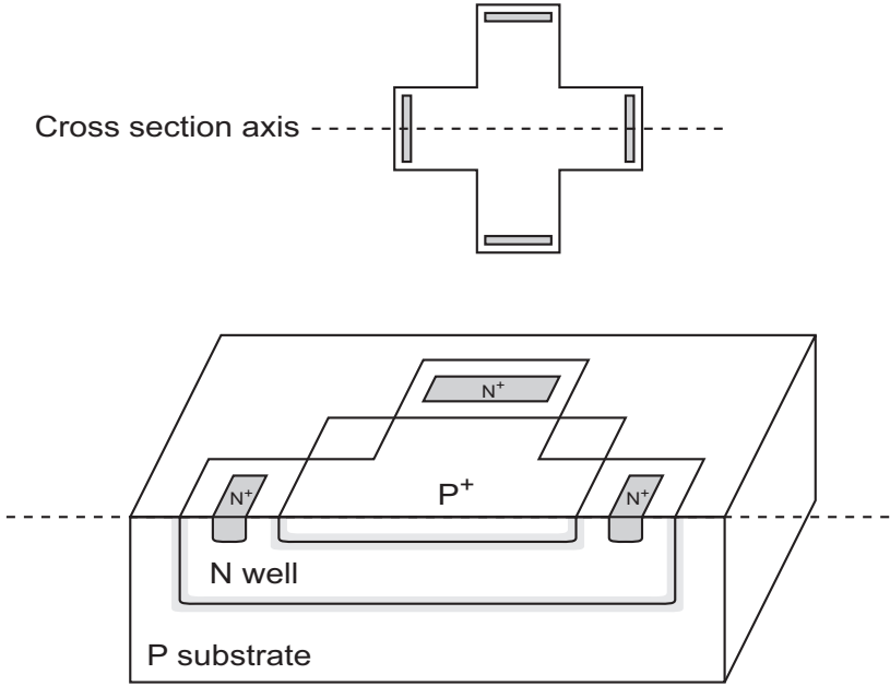
Figure 113. Cross-like Hall sensor implementation in P-substrate CMOS
