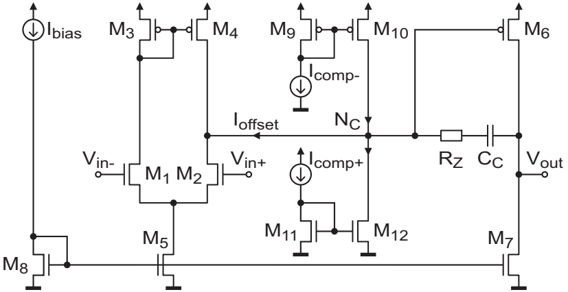
Figure 77. Offset correction by unilateral current injection
