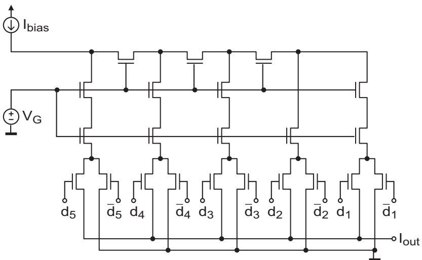
Figure 44. M/3M ladder
