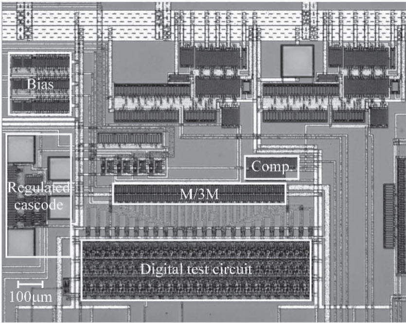
Figure 65. DAC micrograph
