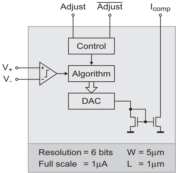
Figure 89. Single-ended compensation component in the schematic editor
