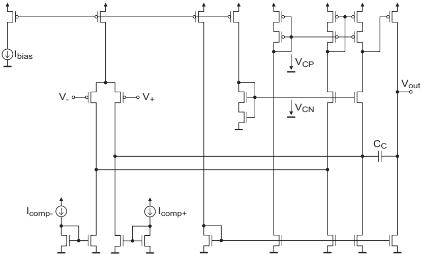
Figure 145. Schematic of the operational amplifier
