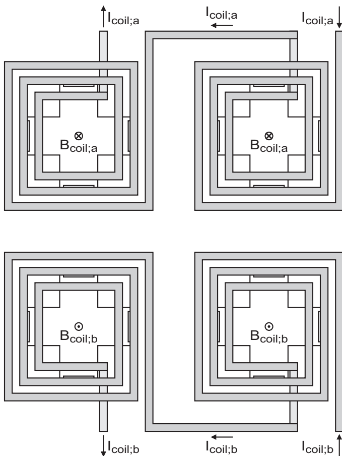
Figure 140. Hall sensor and reference coil array
